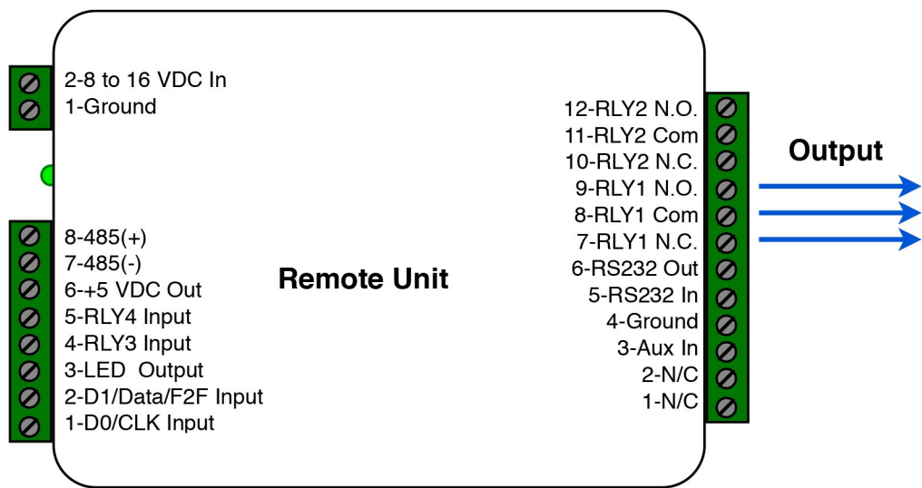
Relay 1 Input and Output
