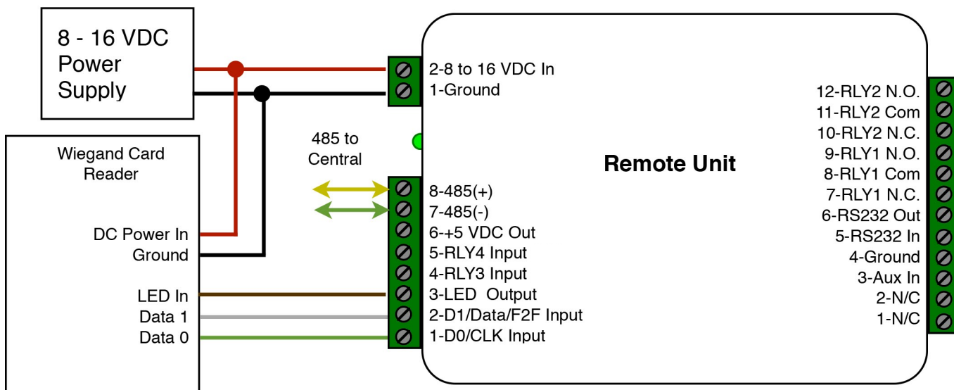
Wiegand Reader with 8-16 Volt power Connections
